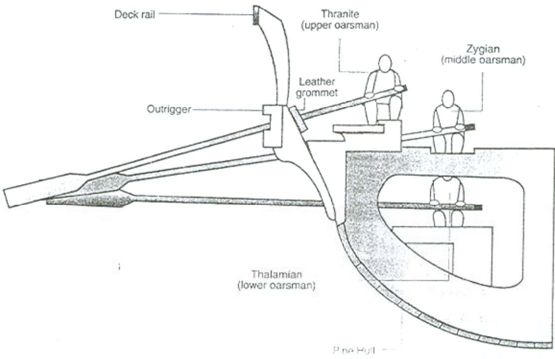
Cross-section of the rowing positions on an ancient Greek trireme
